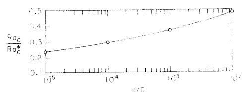
FIG. 2. Critical Rayleigh number vs. d/D for k_f/k_s = 0.133
